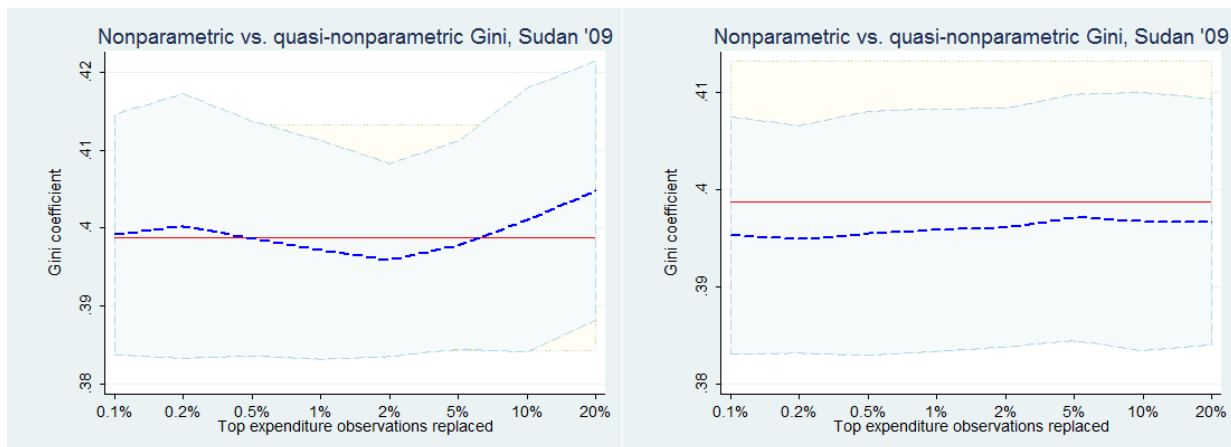
q. Pareto distribution correction, Sudan '09
