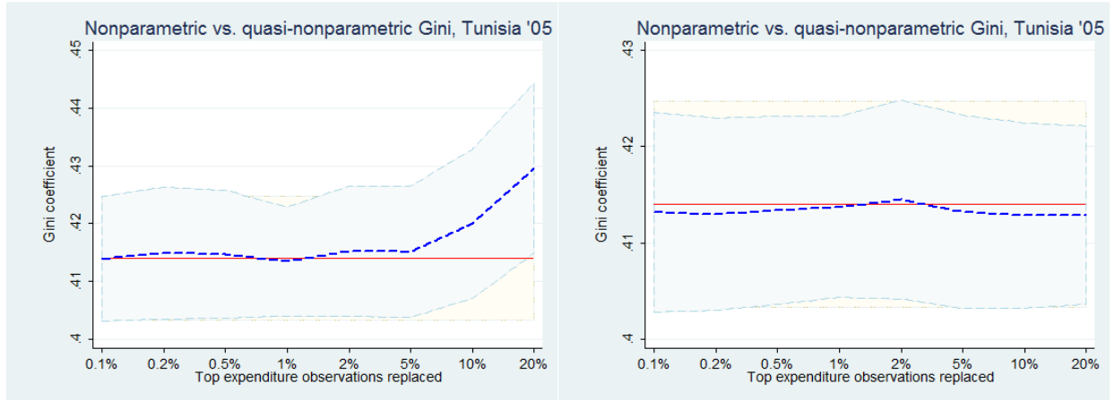
s. Pareto distribution correction, Tunisia '05
