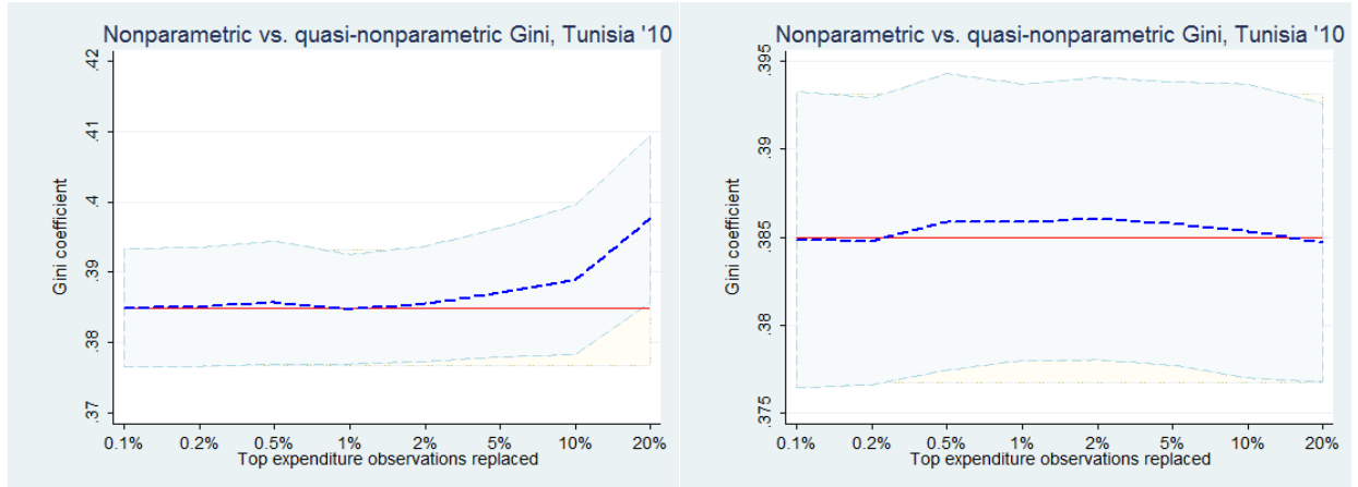
u. Pareto distribution correction, Tunisia '10
