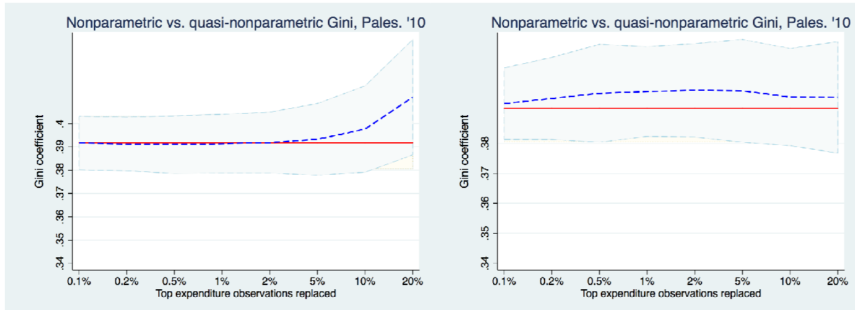
m. Pareto distribution correction, Palestine '10
