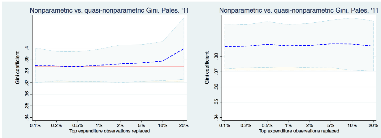
o. Pareto distribution correction, Palestine '11
