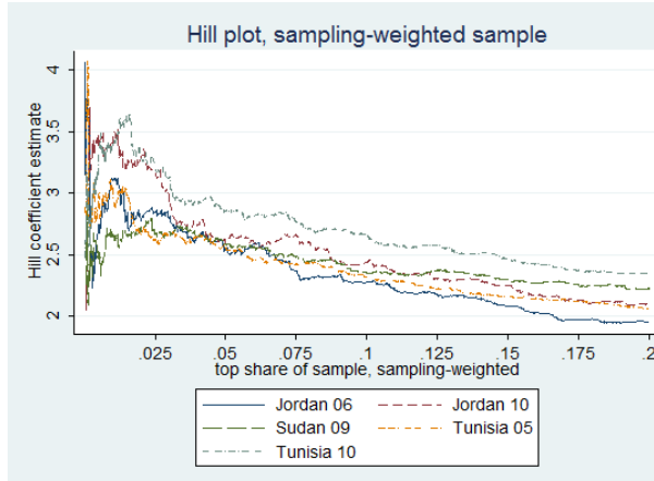
(c) Hill plots: Jordan, Sudan and Tunisia
